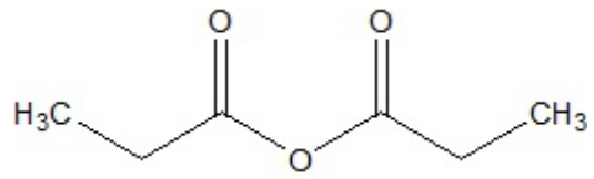
Propionic anhydride
